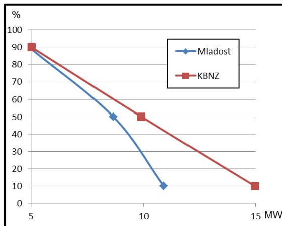
Figure 4: Probability plot for Mladost and KBNZ systems power outputs
