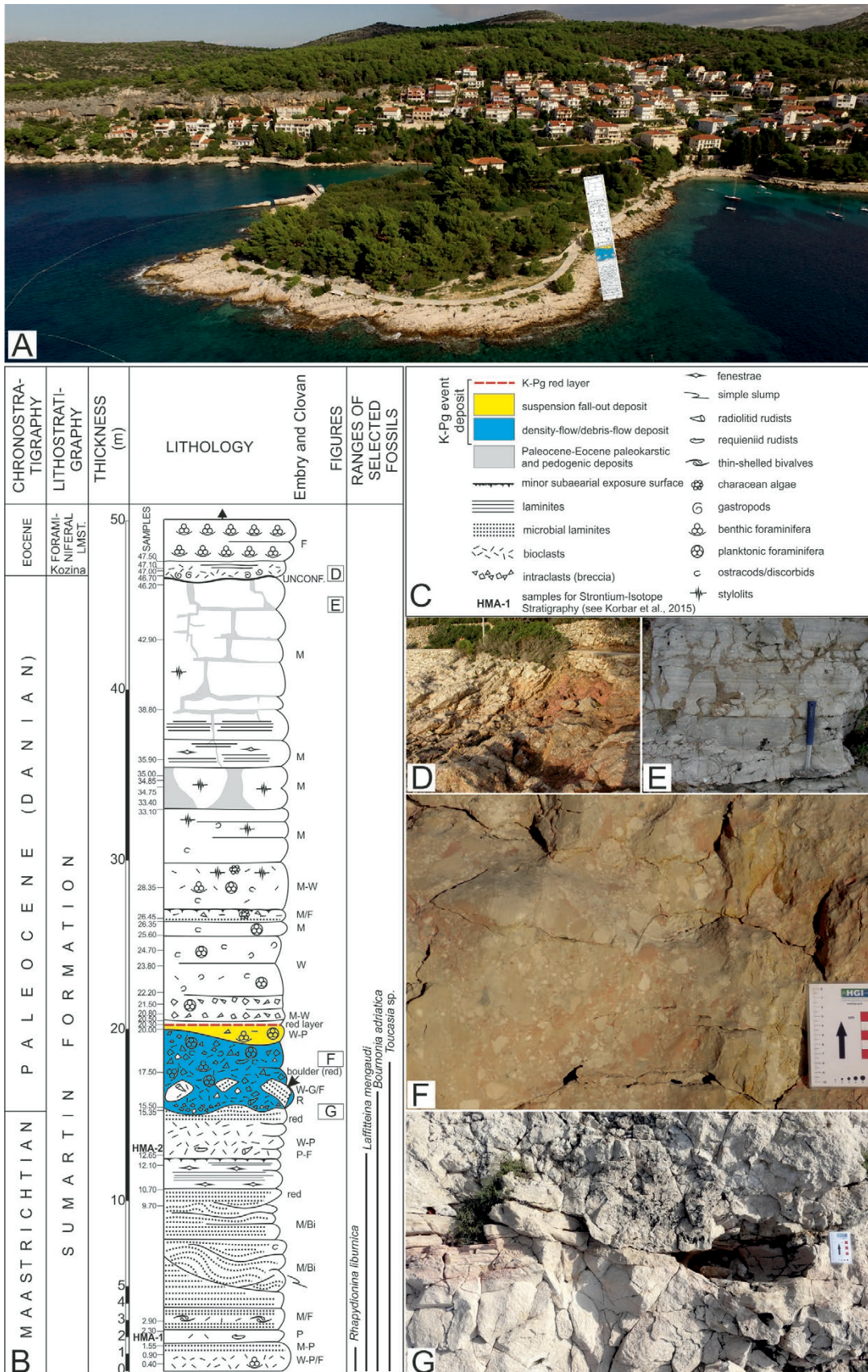
Fig. 11. Hvar K-Pg section at Majerovica – Kovač (see Korbar et al., 2015). A ) Panoramic photograph from the south to Kovač Promontory, Majerovica Cove (right), and Podstine Cove (background left), indicating the position of the measured section. B ) Stratigraphic column Hvar – Majerovica. C ) Legend for B . D ) Palaeocene platform top covered by reddish-brown calcrete and bauxite (right) and the overlying Eocene Foraminiferal Limestones (left). E ) Discontinuity surfaces and palaeokarst infillings by calcrete within the Palaeocene succession of peritidal carbonates (see Brlek et al., 2014). F ) K-Pg boundary event-bed (tsunamiite?): polymictic, chaotic carbonate breccia characterized by abundant muddy matrix. G ) K-Pg boundary: uneven erosional contact of the underlying reddish microbial peritidal laminites and the overlying chaotic carbonate breccia.
